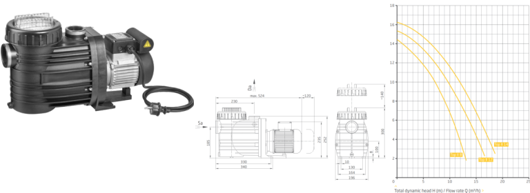
BADU Top II 14m3/h H=8m 0,65kW/230V
